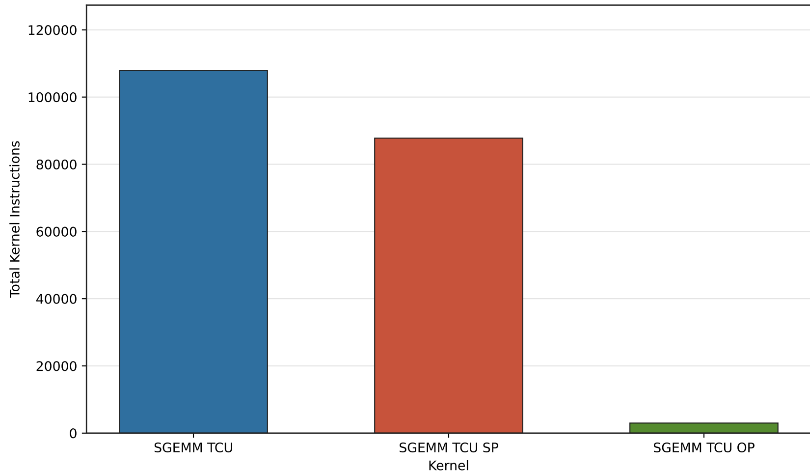
FP16 Total Kernel Instructions by Kernel MxNxK=128x128x512
