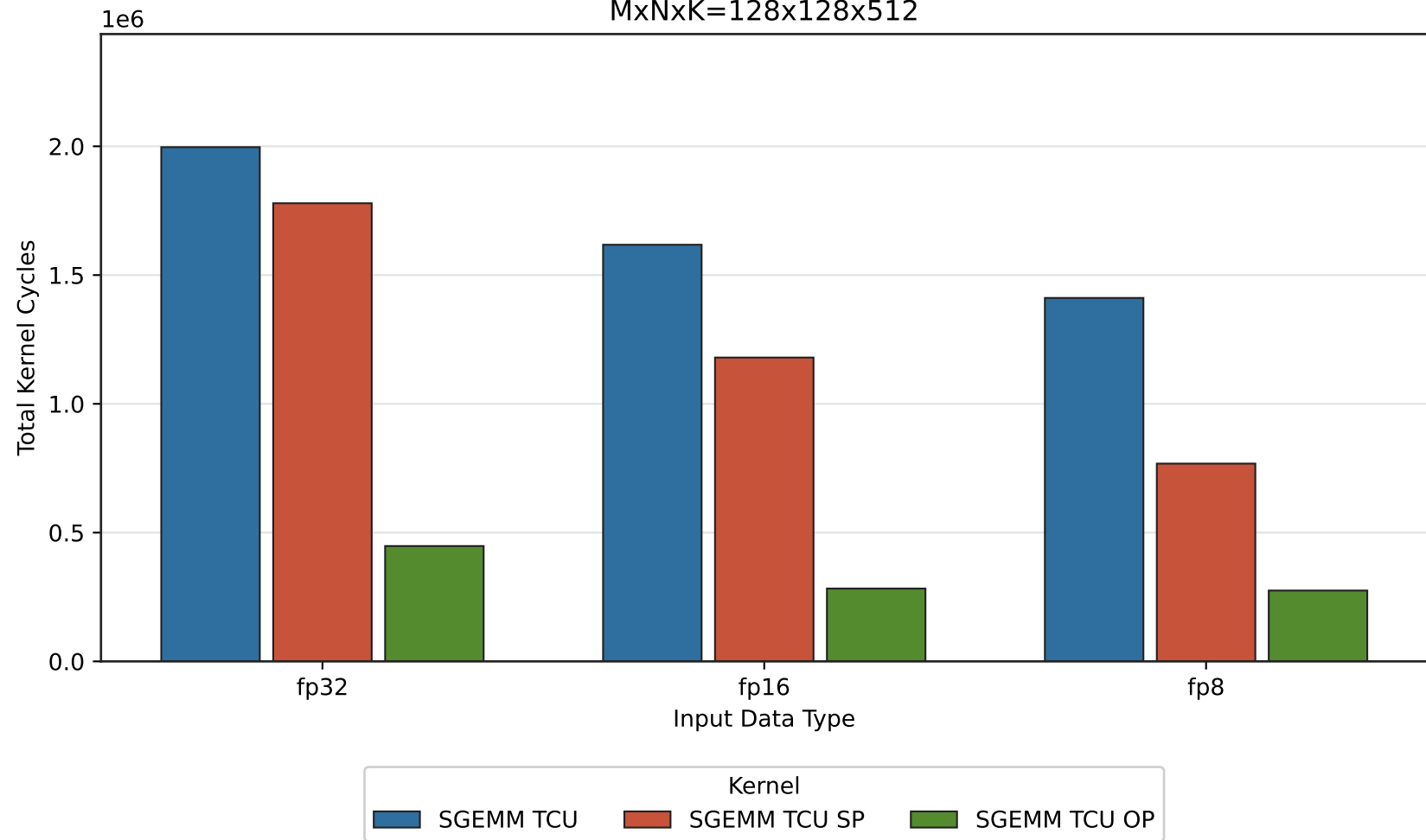
Total Kernel Cycles by Input Data Type MxNxK=128x128x512
