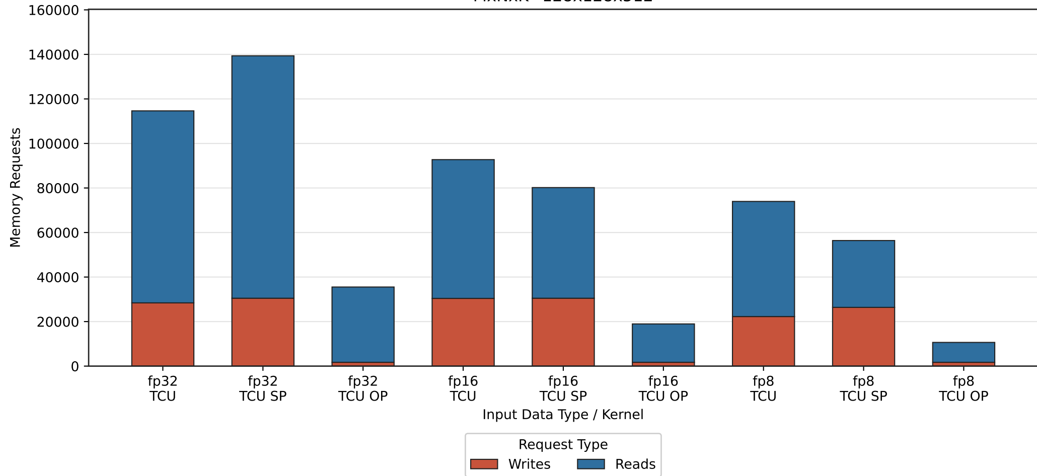
Memory Requests by Input Data Type and Kernel MxNxK=128x128x512
