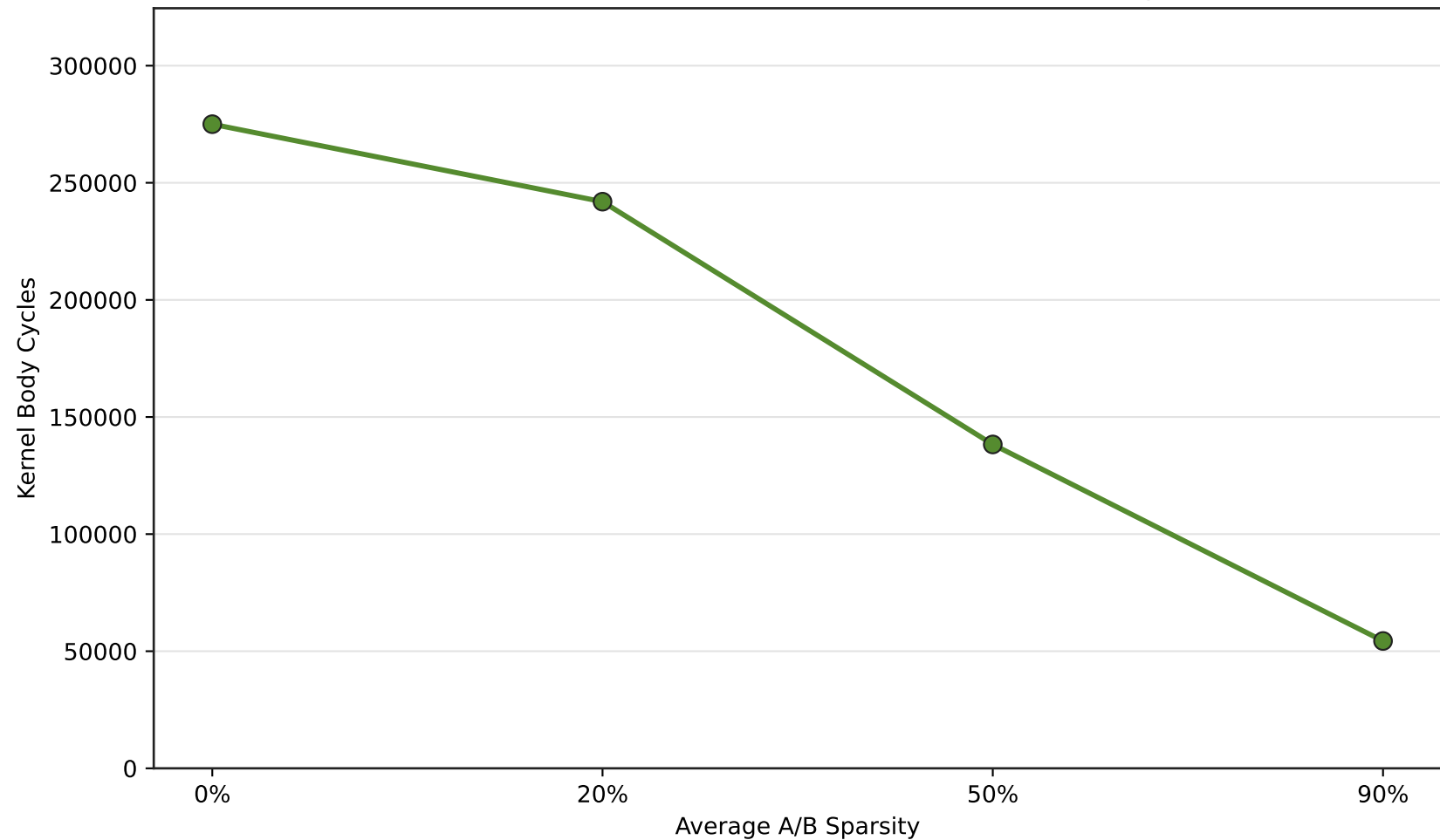
Kernel Body Cycles by Sparsity MxNxK=128x128x512, Kernel=SGEMM TCU OP, It=fp8
