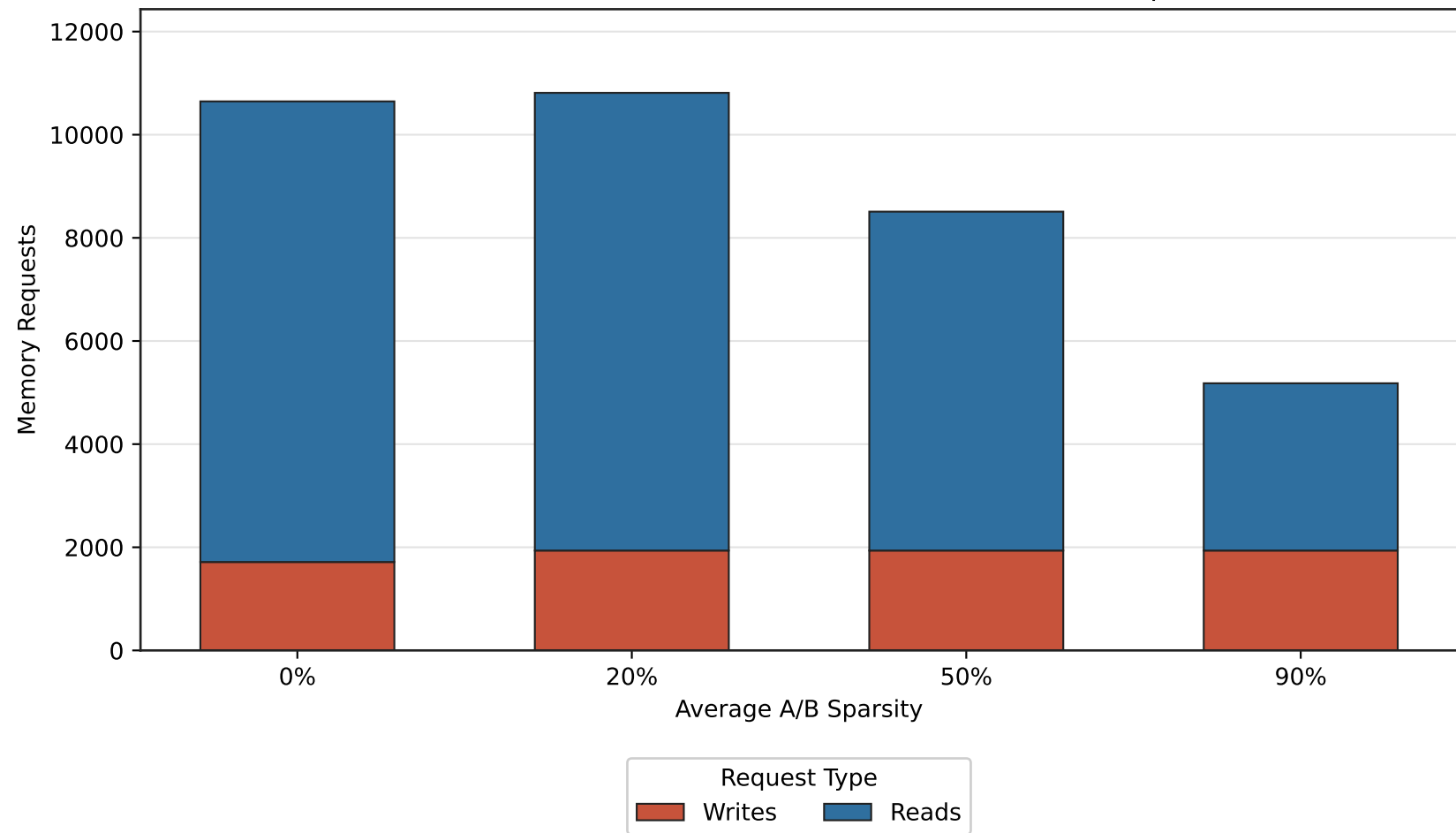
Memory Requests by Sparsity MxNxK=128x128x512, Kernel=SGEMM TCU OP, It=fp8
