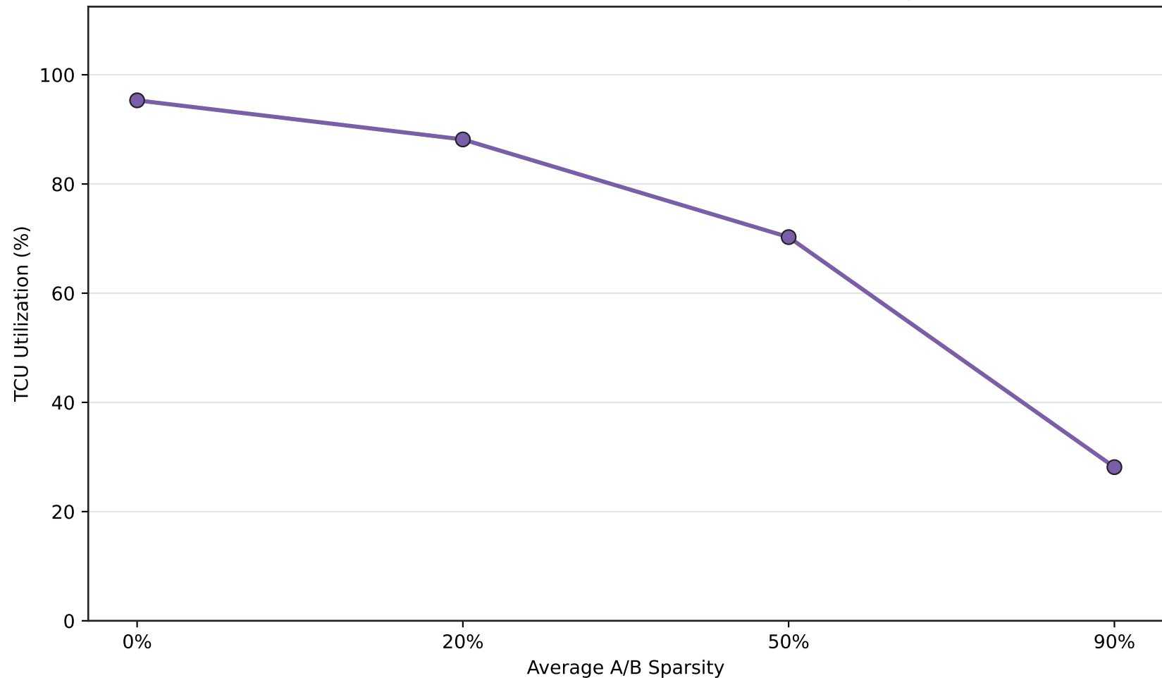
TCU Utilization by Sparsity MxNxK=128x128x512, Kernel=SGEMM TCU OP, It=fp8
