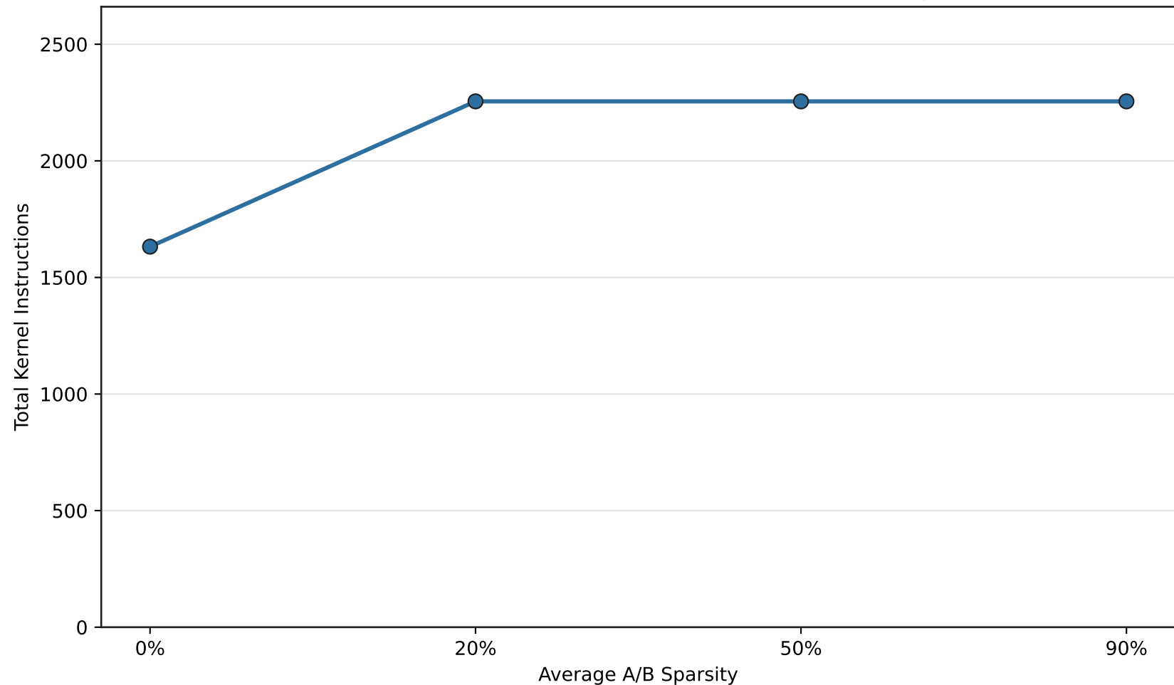
Total Kernel Instructions by Sparsity MxNxK=128x128x512, Kernel=SGEMM TCU OP, It=fp8
