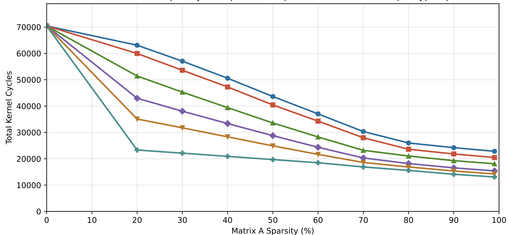
SGEMM TCU OP Sparsity Sweep - Matrix operation: 64x64x512, Input type: fp8
