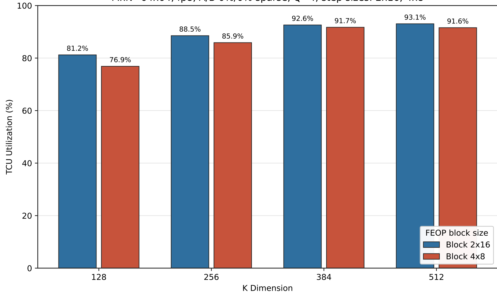
TCU Utilization Increases with Larger K MxN=64x64, fp8, A/B 0%/0% sparse, Q=4, step sizes: 2x16, 4x8
