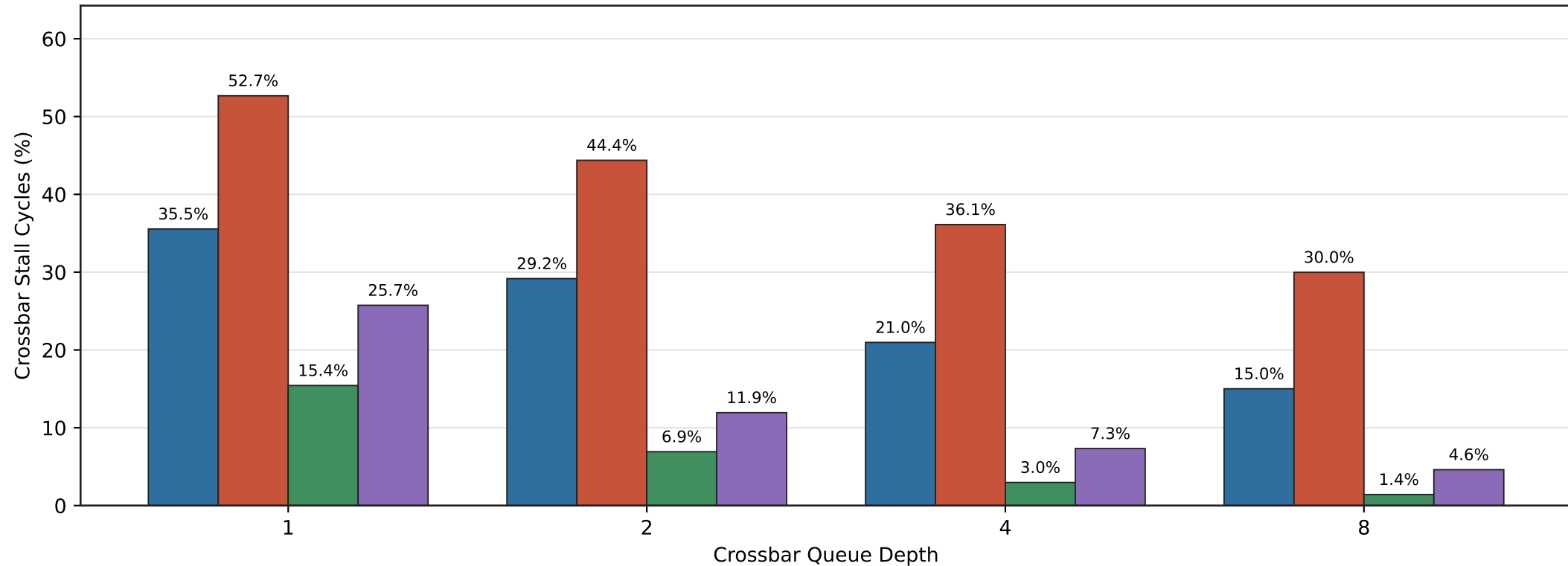
Queue Depth Effect on Crossbar Stalls - 64x64x512, fp8
