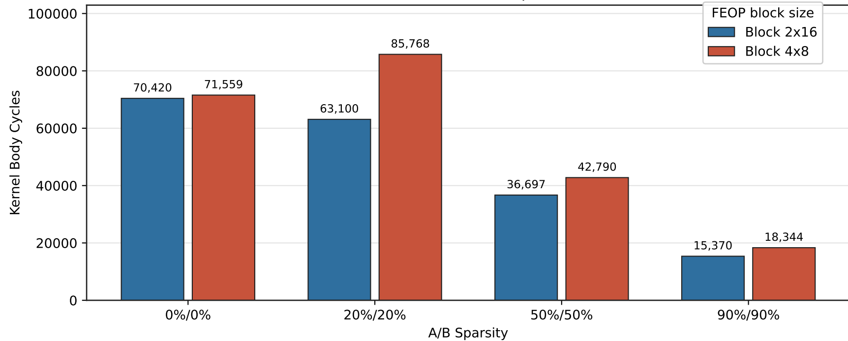
Kernel Cycles by Sparsity and FEOP Block Size MxNxK=64x64x512, fp8, Q=4
