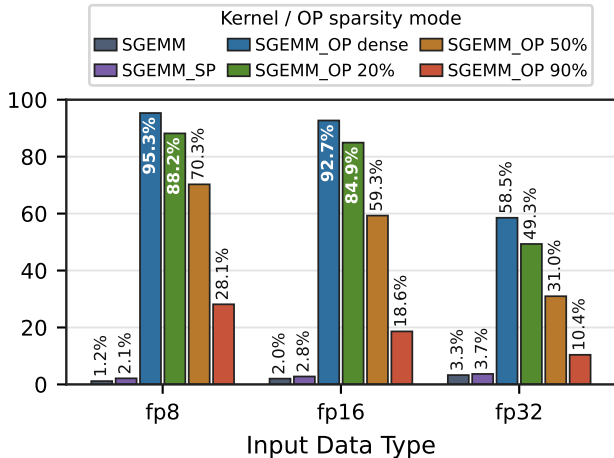
TCU Multiplier Utilization (%)
