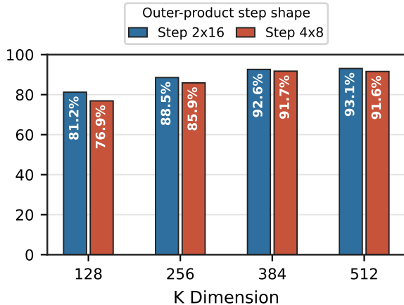
TCU Multiplier Utilization (%)
