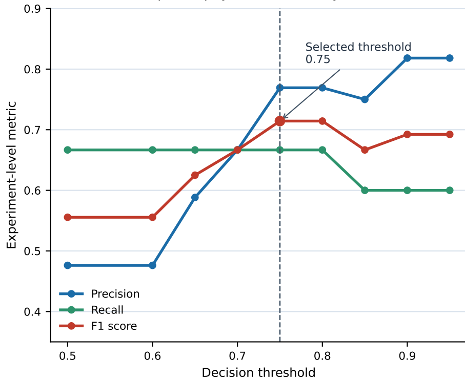
Threshold sweep with physics-consistency filter
