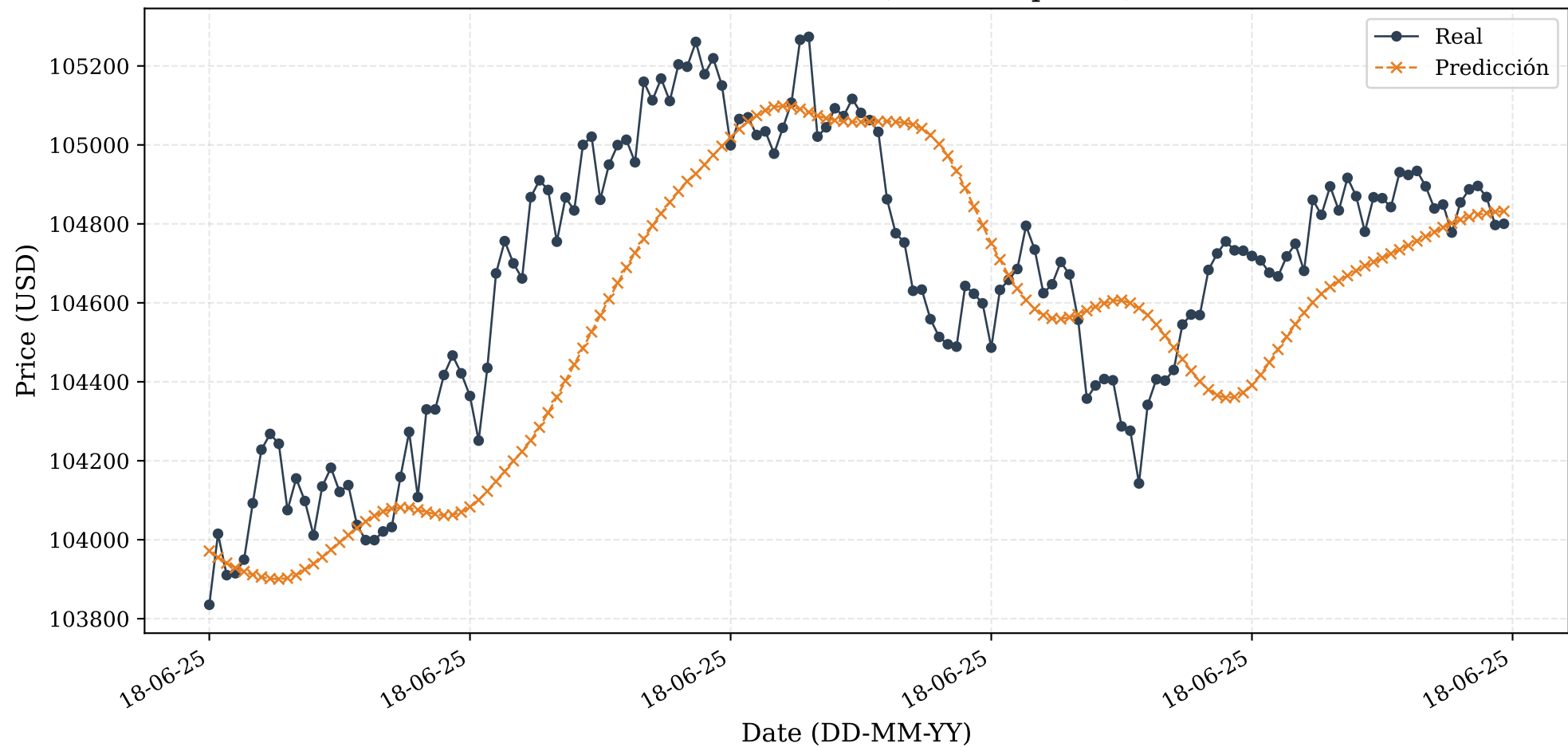
Prediction Detailed (Last 150 points)
