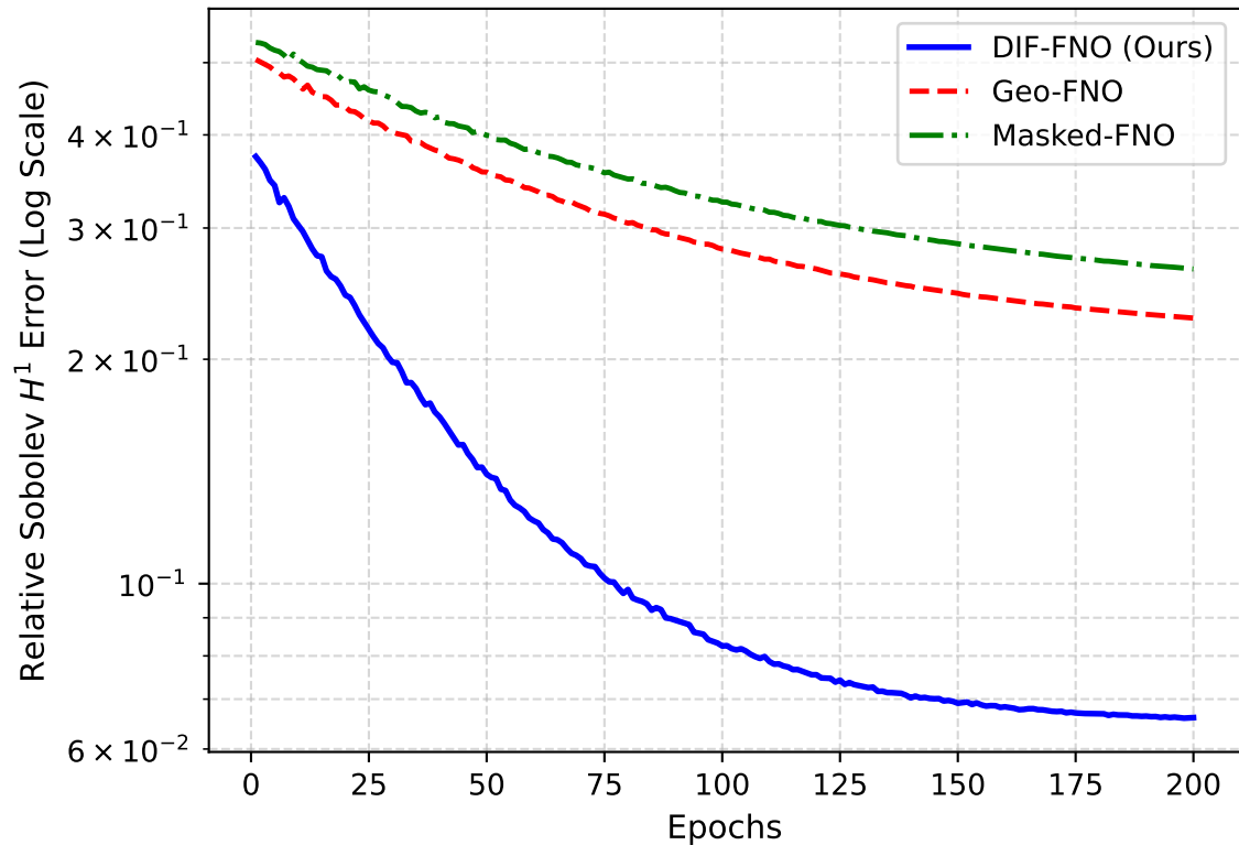
Test Sobolev H^1 Convergence Rate
