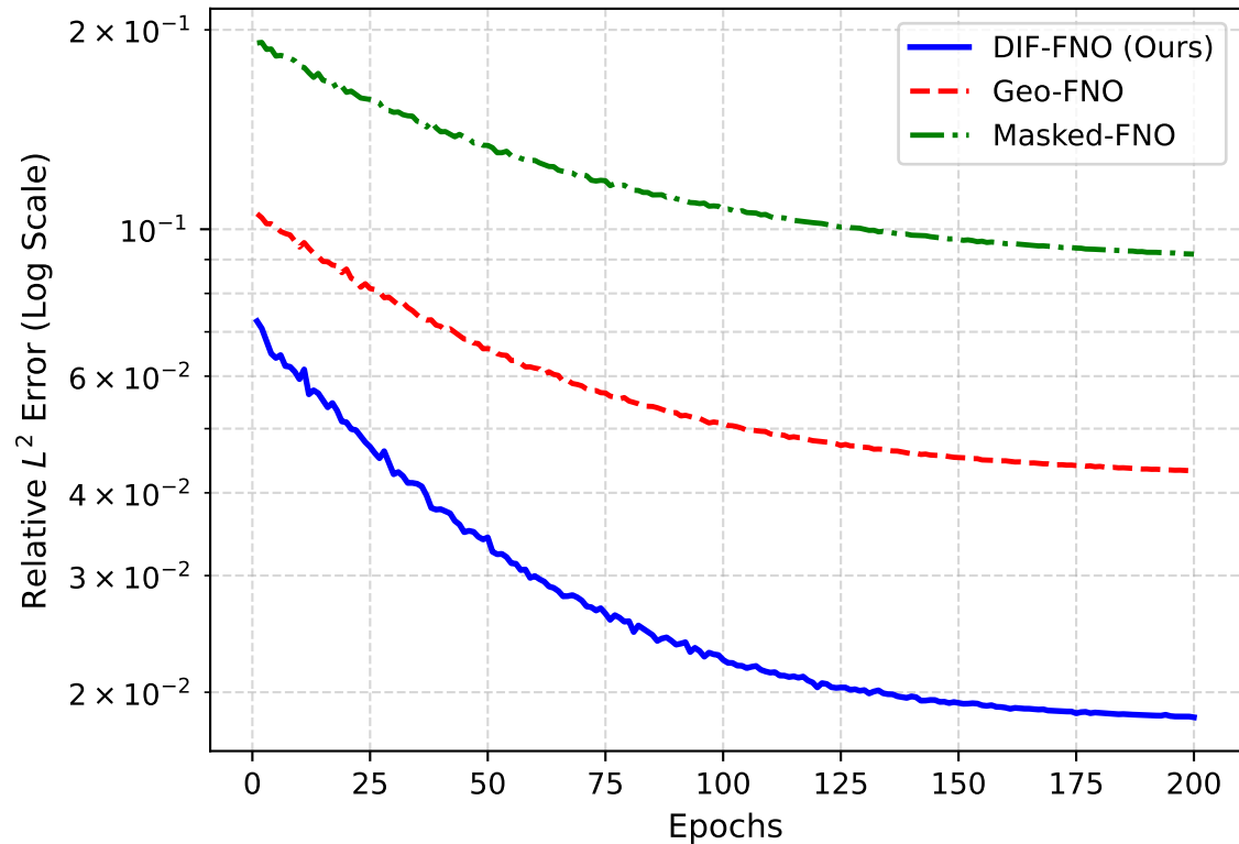
Test L^2 Convergence Rate
