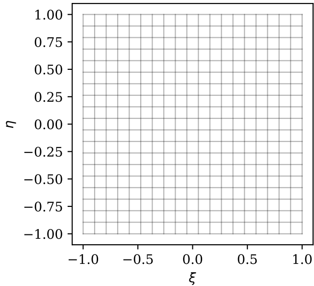
Latent Reference Domain \Omega_l
