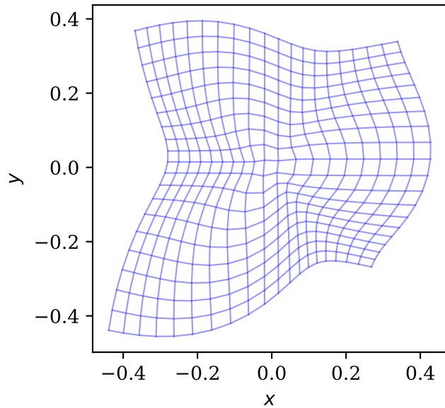
Physical Domain \Omega_p ( \det(J) > 0 )
