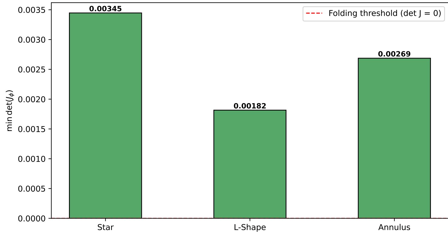
DIF-FNO v4: Minimum Jacobian Determinant \min \det(J_\phi) > 0
