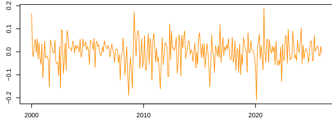
Stock market – Stationary
