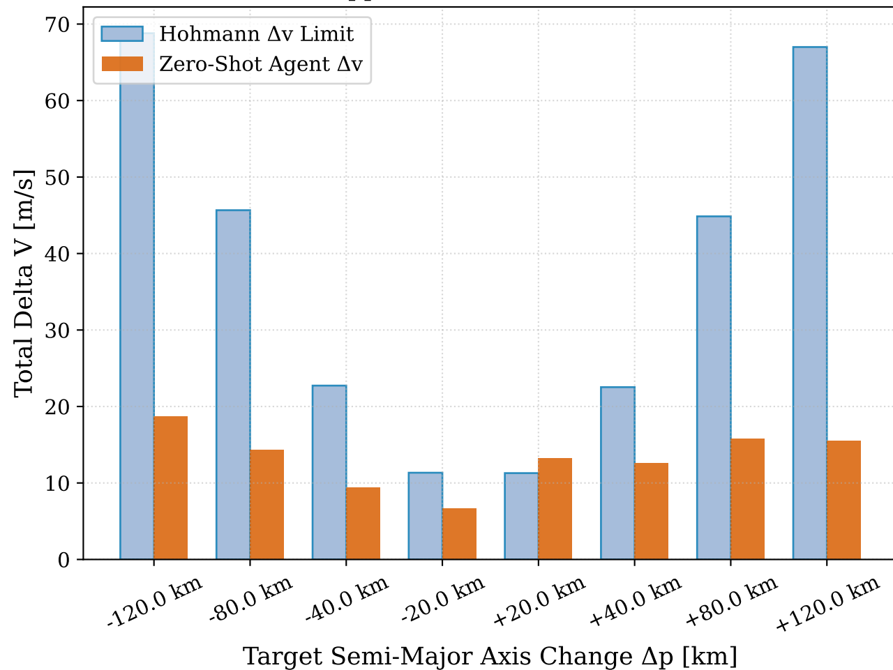
(a) Total Applied Delta V vs Hohmann Limit
