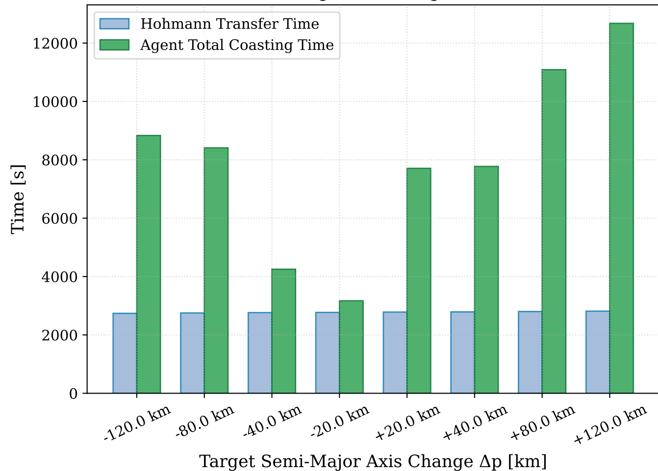
(b) Transfer Time: Agent Coasting vs Hohmann Limit
