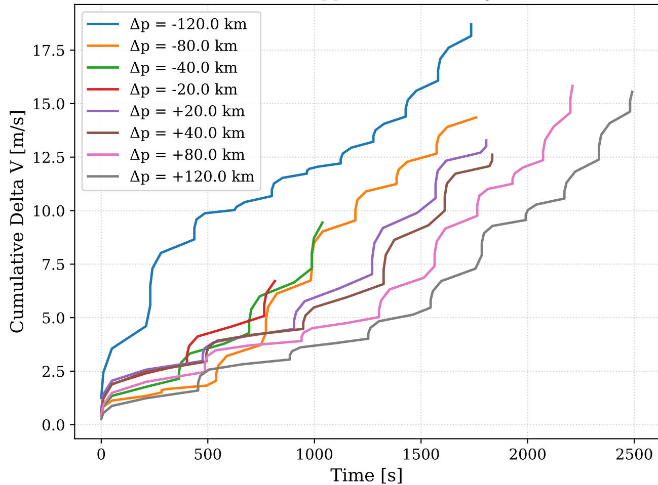
(a) Cumulative Applied Delta V Trajectories
