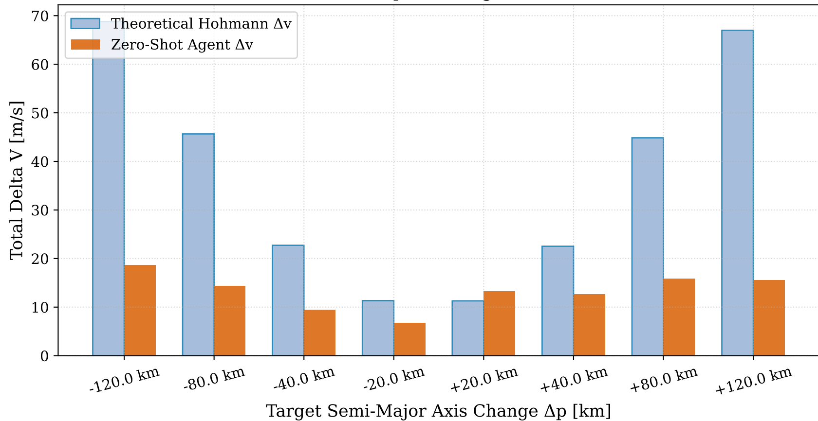
Zero-Shot Delta V Comparison: Agent vs Hohmann Limit
