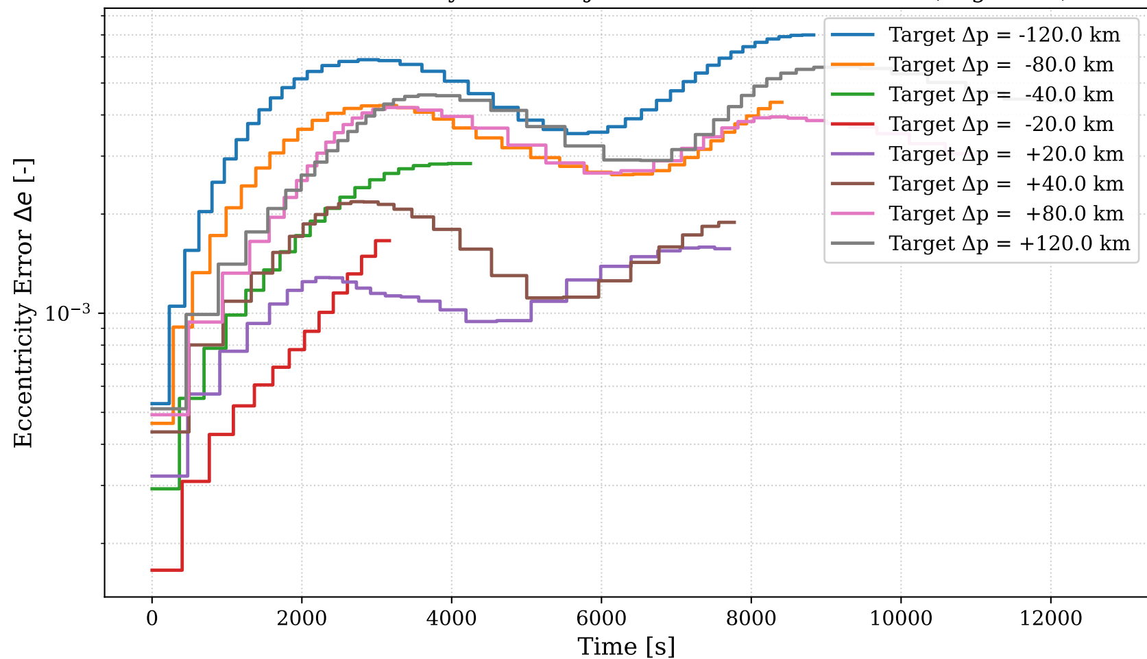
Zero-Shot Eccentricity Error Trajectories Across Test Orbits (Log Scale)
