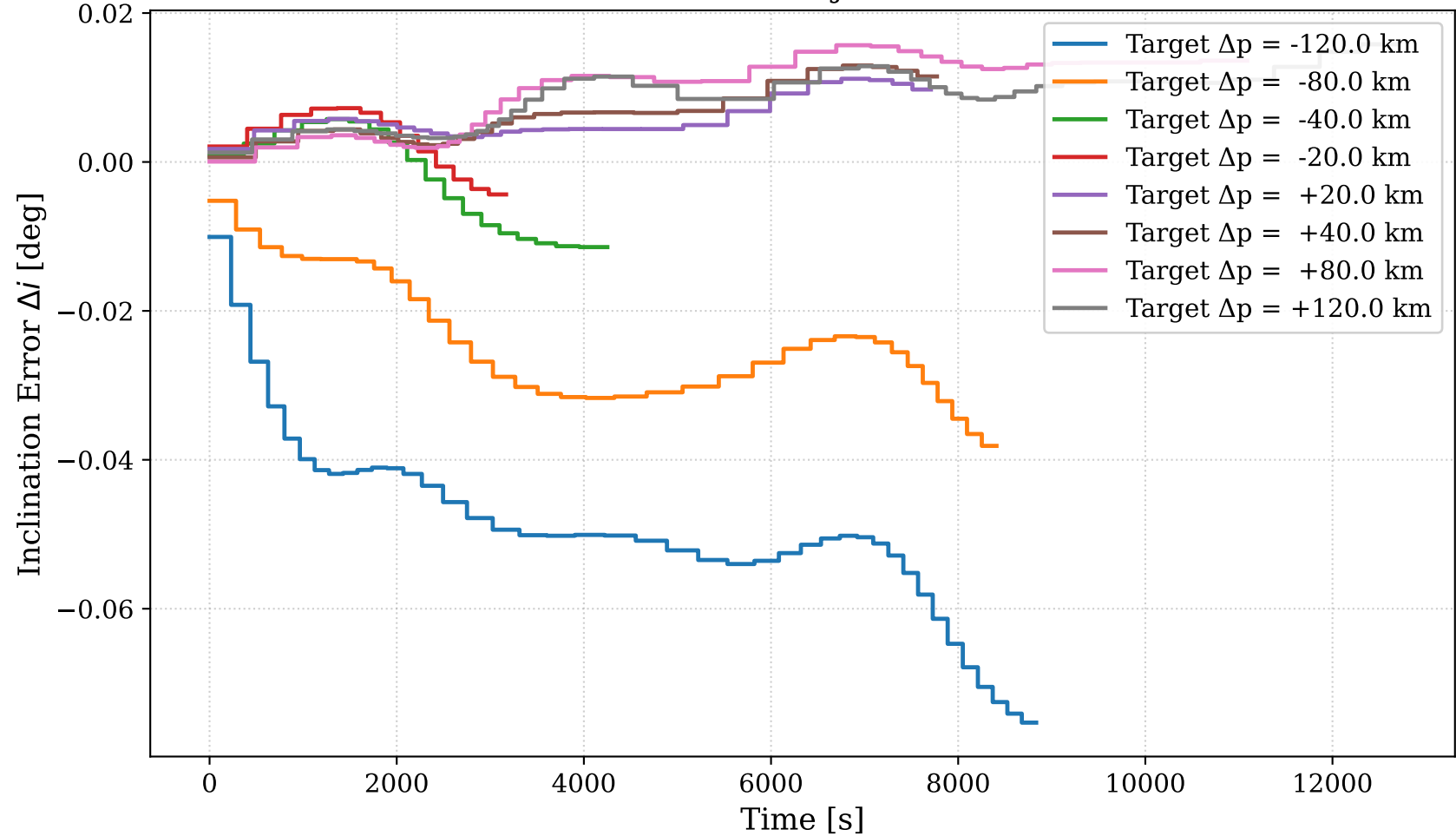
Zero-Shot Inclination Error Trajectories Across Test Orbits
