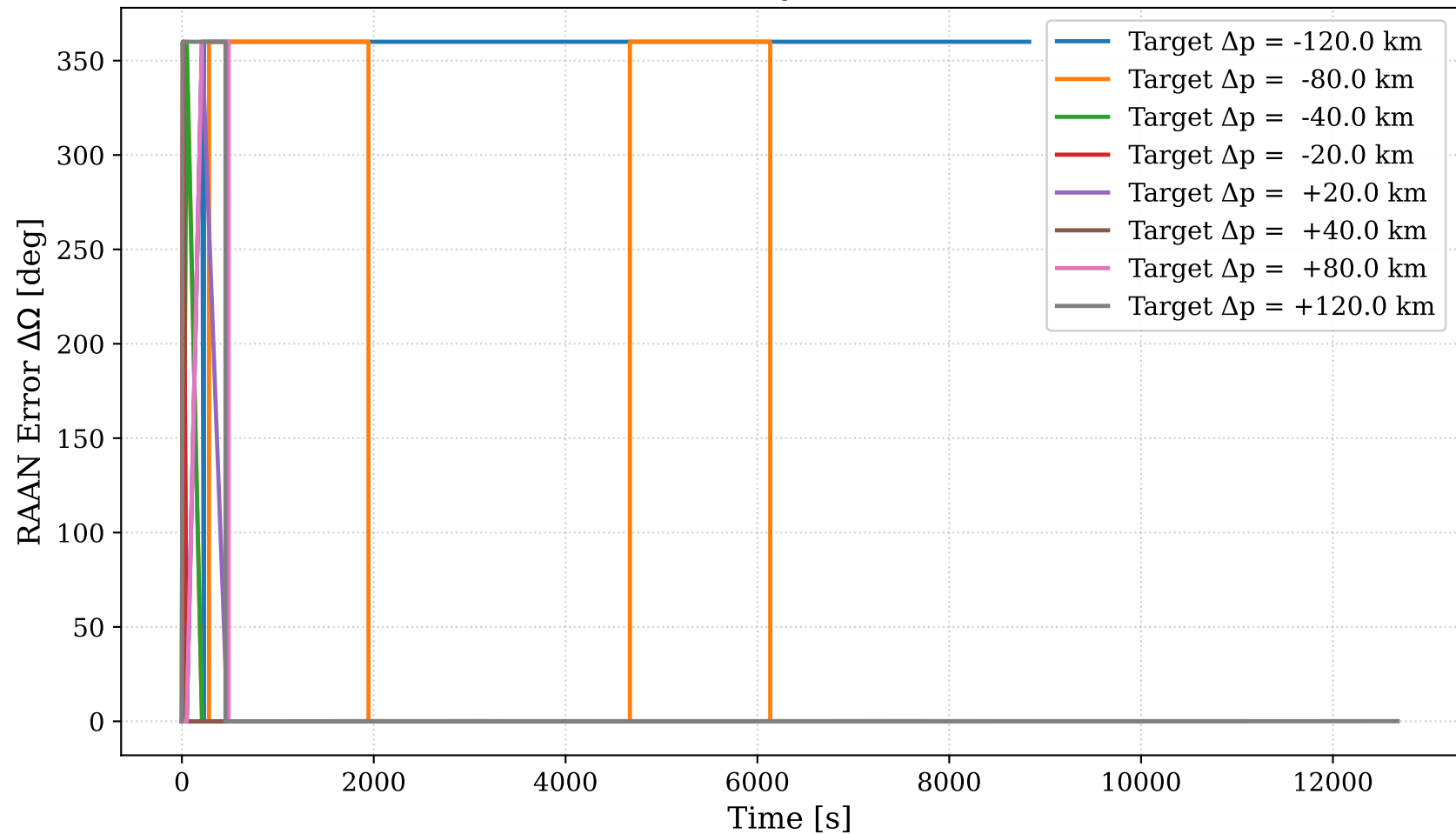
Zero-Shot RAAN Error Trajectories Across Test Orbits
