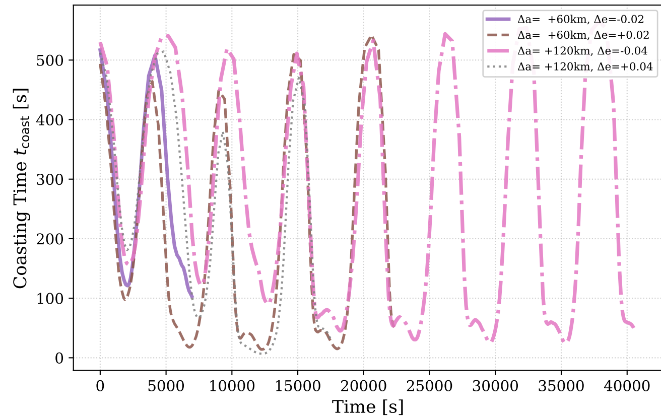
Coasting Duration Profile ( t_{\text{coast}} ) ( \Delta a > 0 )
