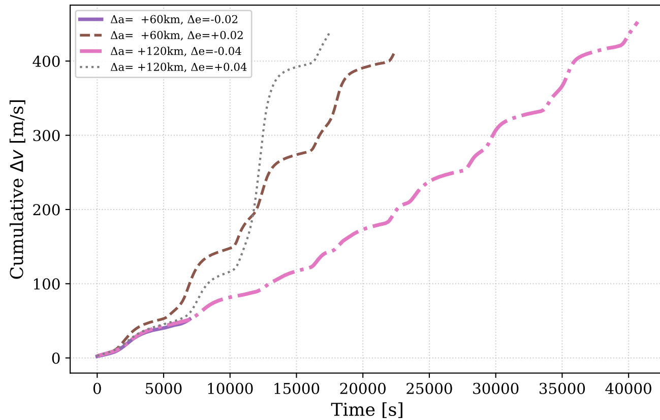
Cumulative \Delta v Profile ( \Delta a > 0 )
