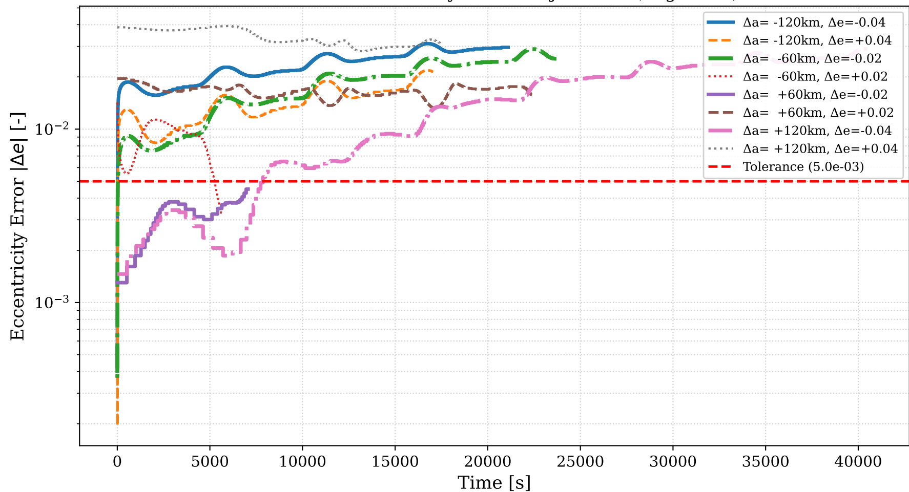
Zero-Shot Eccentricity Error Trajectories (Log Scale)
