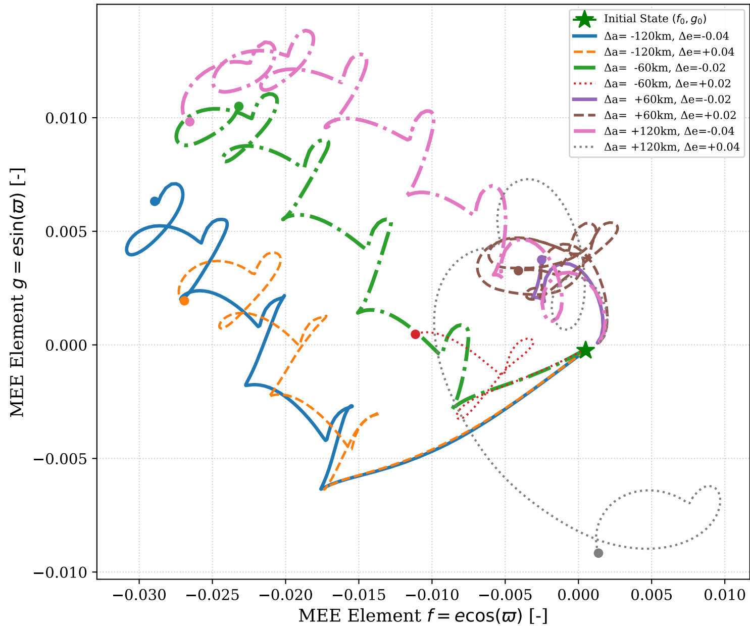
MEE Eccentricity Phase Plane Trajectories ( f, g )
