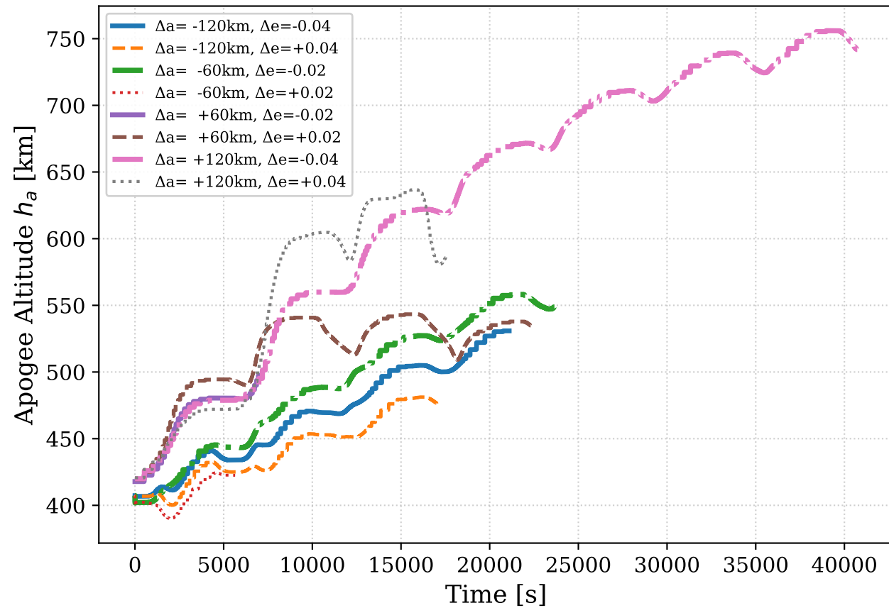
Apogee Altitude Evolution ( h_a )
