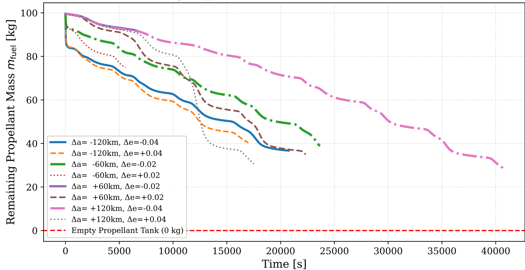
Remaining Propellant Mass Over Time Across Test Orbits
