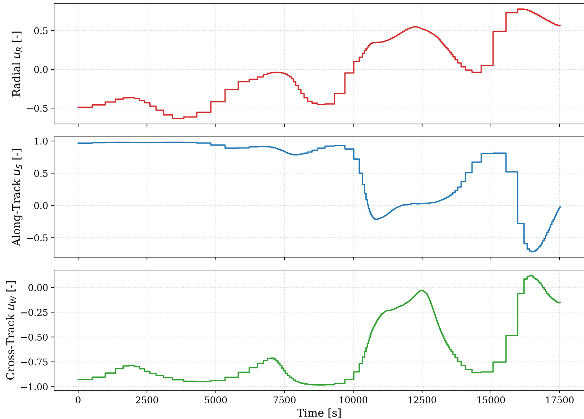
RSW Thrust Vector Breakdown ( \Delta a = +120 km, \Delta e = +0.04 )
