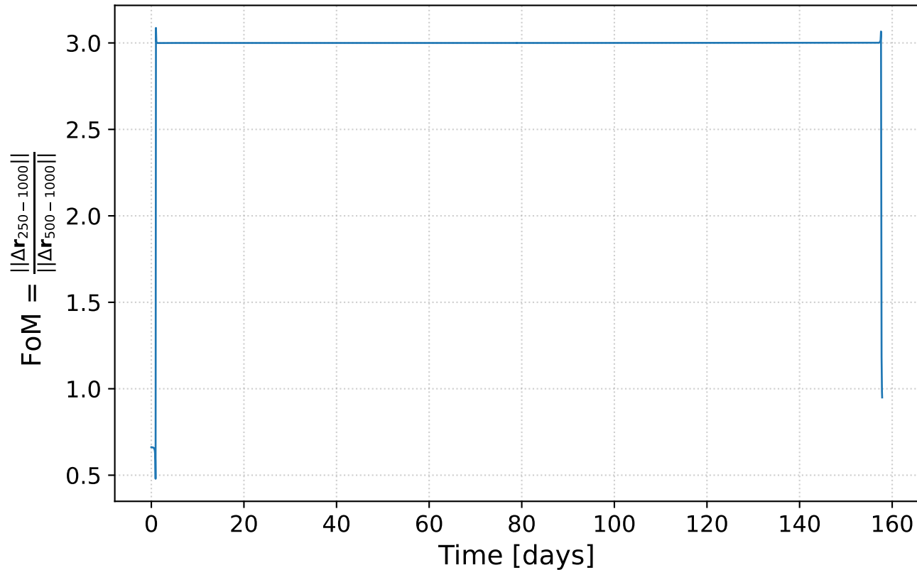
Figure of Merit: Impact of Spacecraft Mass on Trajectory (Case IV)
