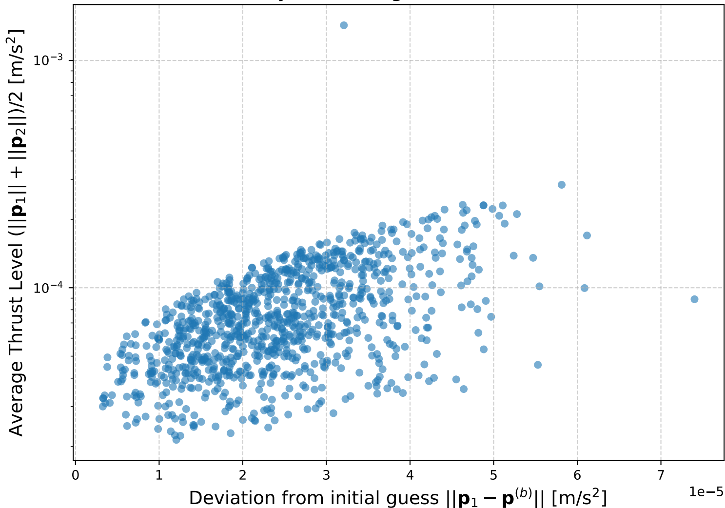
Monte Carlo Analysis: Average Thrust vs. Deviation (Q4d)
