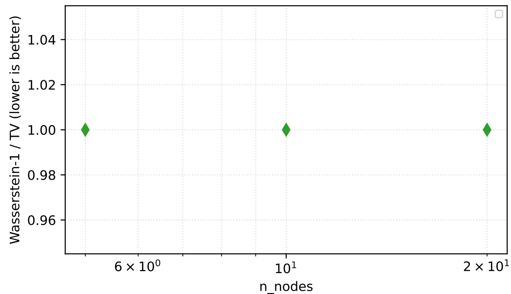
continuous_nongauss
