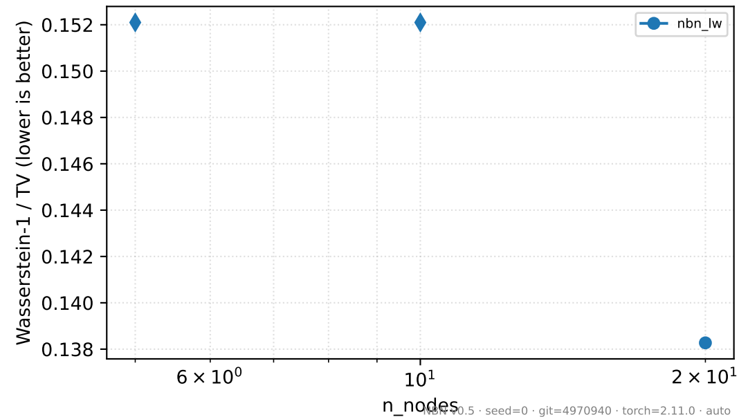
hybrid
