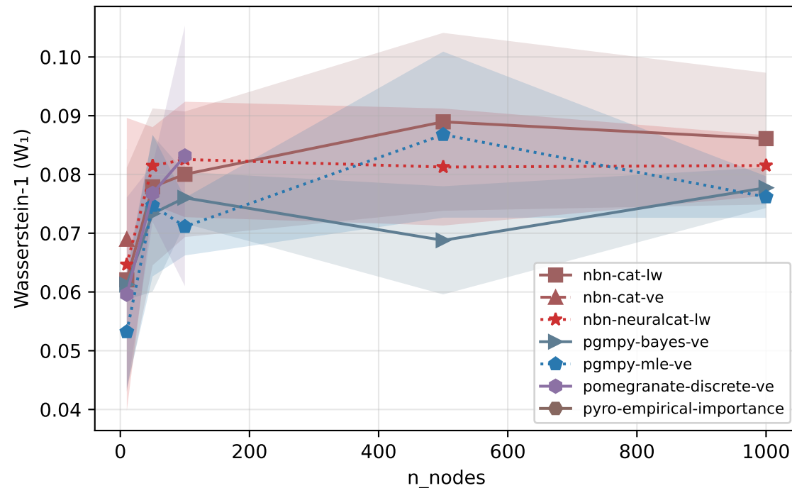
continuous_nongauss
