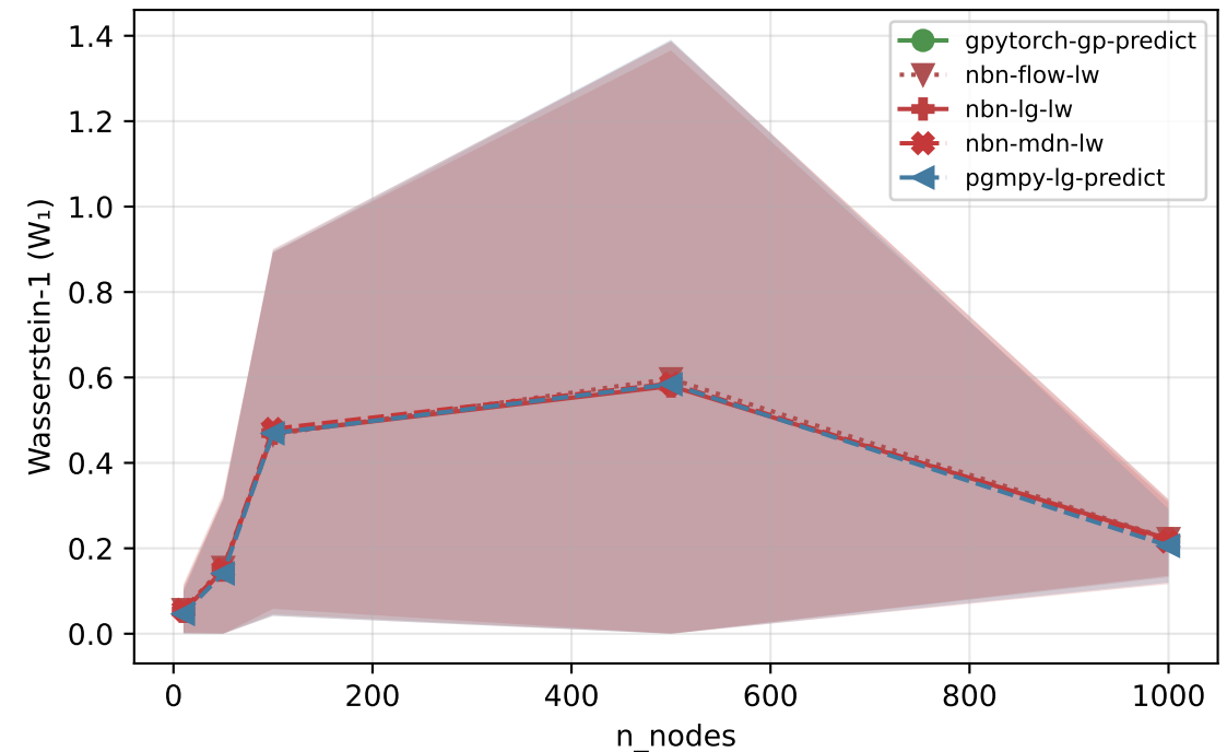
hybrid
