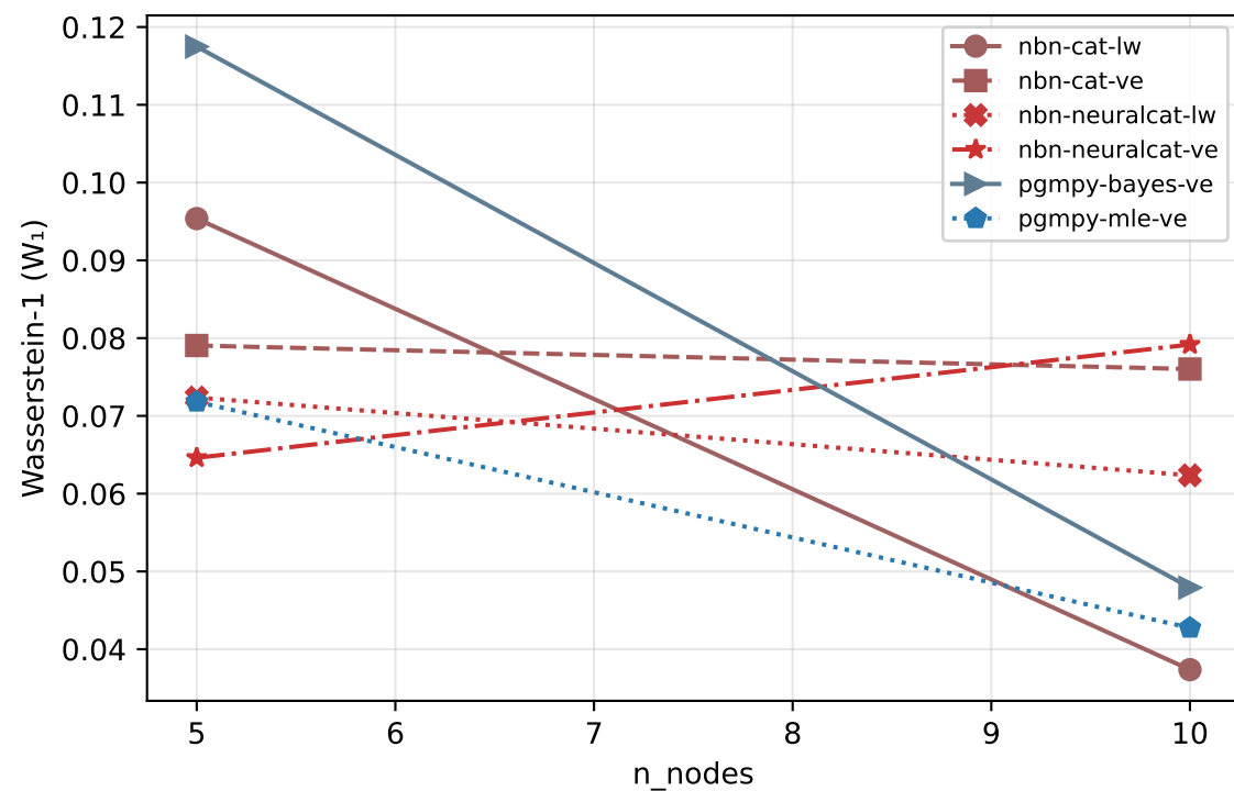
continuous_nongauss
