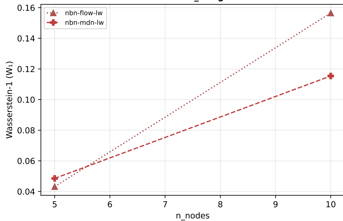
continuous_nongauss
