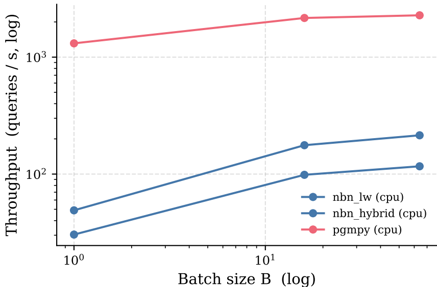
Inference throughput vs batch size
