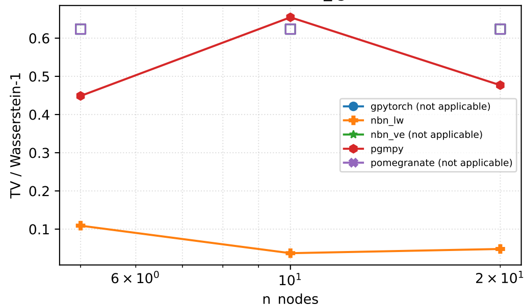
hybrid
