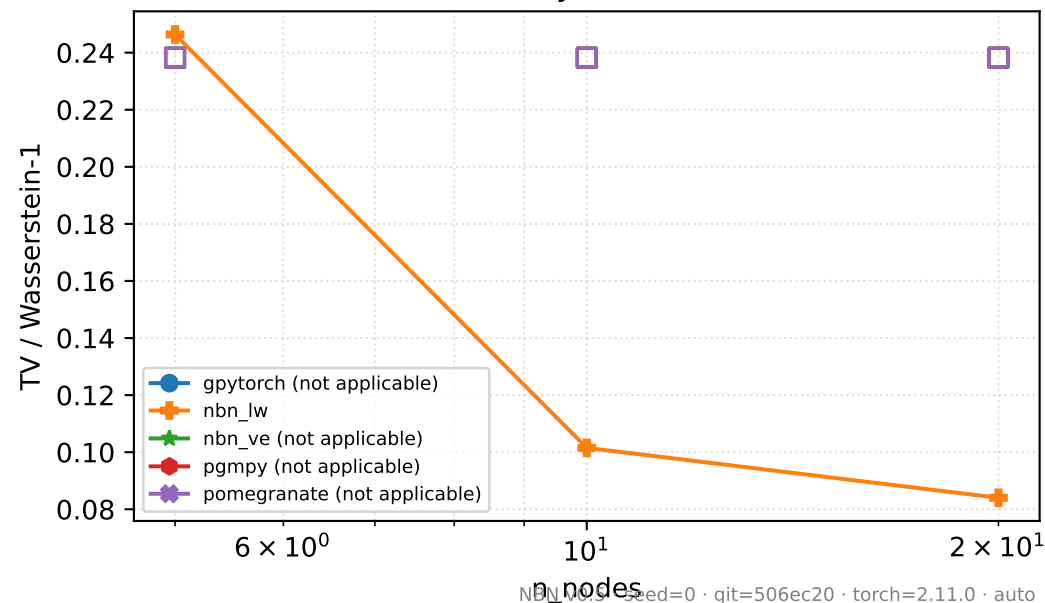
hybrid
