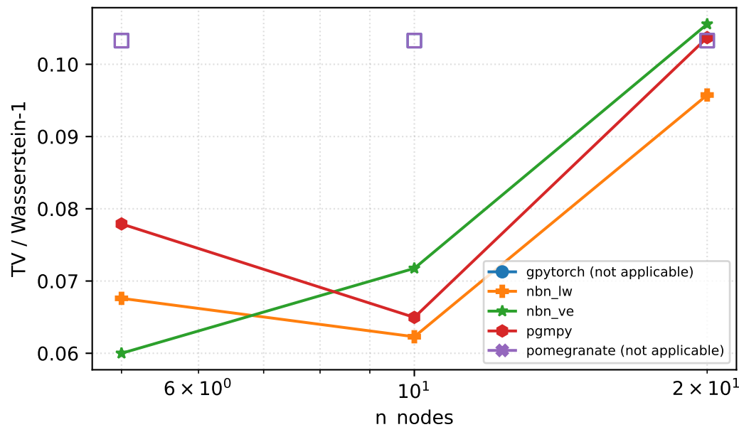
continuous_nongauss
