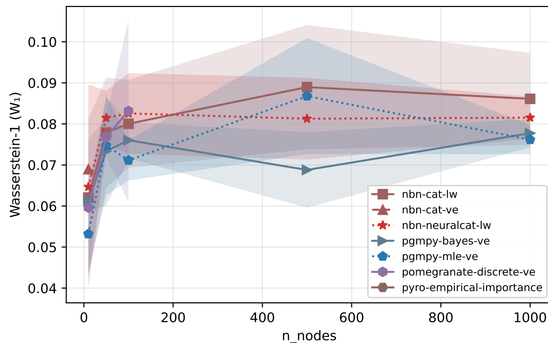
continuous_nongauss
