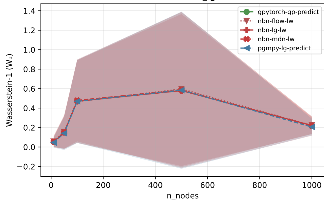
hybrid
