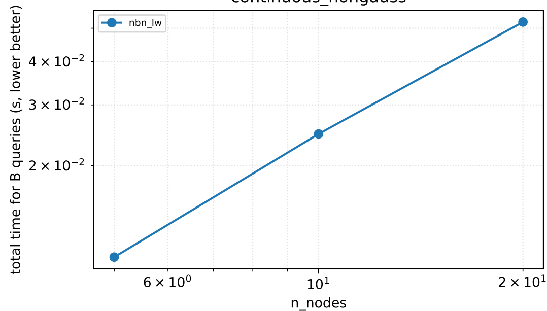
continuous_nongauss
