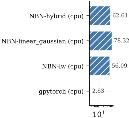
(c) Hybrid (synthetic-50) — speed
