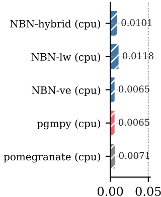
(b) Discrete (alarm) — TV
