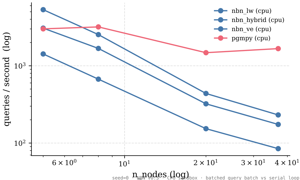
Batched throughput on bnlearn ladder (B=1024, CPU)
