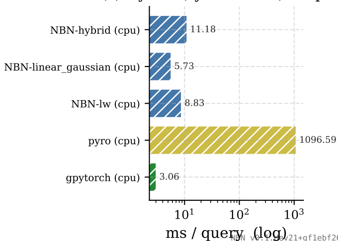
(c) Hybrid (synthetic-50) — speed
