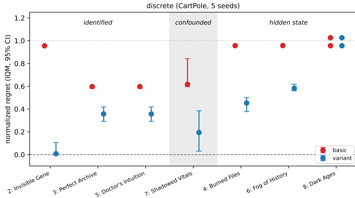
Regret by identification regime, per anchor (SEPARATE y-axes - heights NOT cross-anchor comparable; cells are not a difficulty axis)
