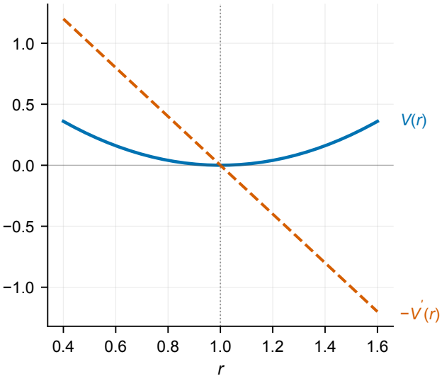
radial confinement
