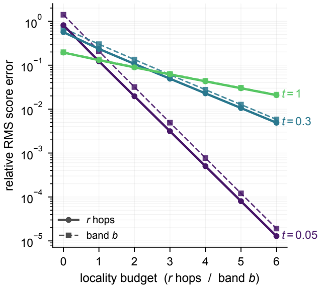
each extra hop buys a constant factor
