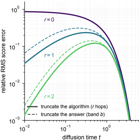
cost of locality across the diffusion
