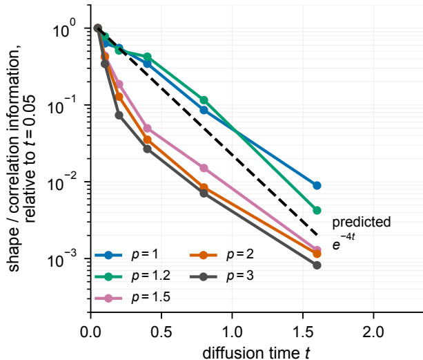
(b) the predicted contrast, five shapes
