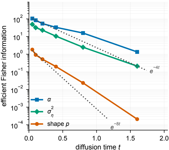
(a) Laplace innovations, p = 1
