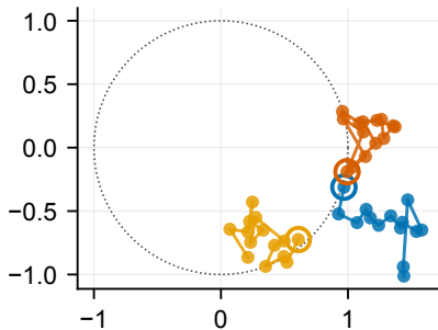
co-rotating frame y_k
