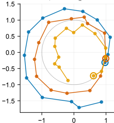
laboratory frame z_k
