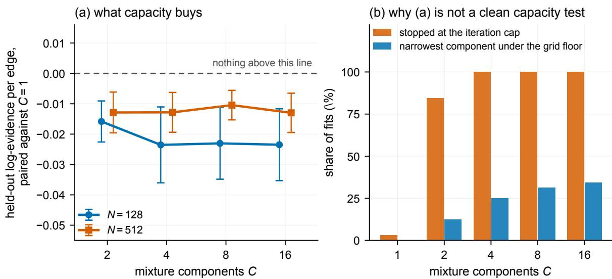
Figure 10.3: (a) Held-out log-evidence per edge, paired within seed against C = 1 : no tested capacity improves on a single Gaussian innovation at either size, and at N = 128 the C = 16 deficit against C = 8 is resolved against zero. (b) Why (a) is not a clean capacity test: the share of fits stopped at the iteration cap, and with a narrowest component under the grid's resolution floor, both climb steeply with C .
