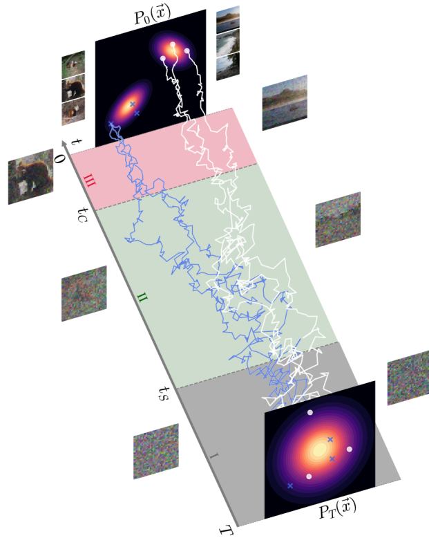
Figure 2.6: The two crossover times below, illustrated on a two-dimensional Gaussian-mixture example. Trajectories destined for different classes are indistinguishable above the speciation time t_S (regime I); between t_S and the collapse time t_C they commit to a class without yet matching any training point (regime II, where a model genuinely generalises); below t_C they are captured by a single training example (regime III). Reproduced from Biroli et al. (2024), their Figure 1.
