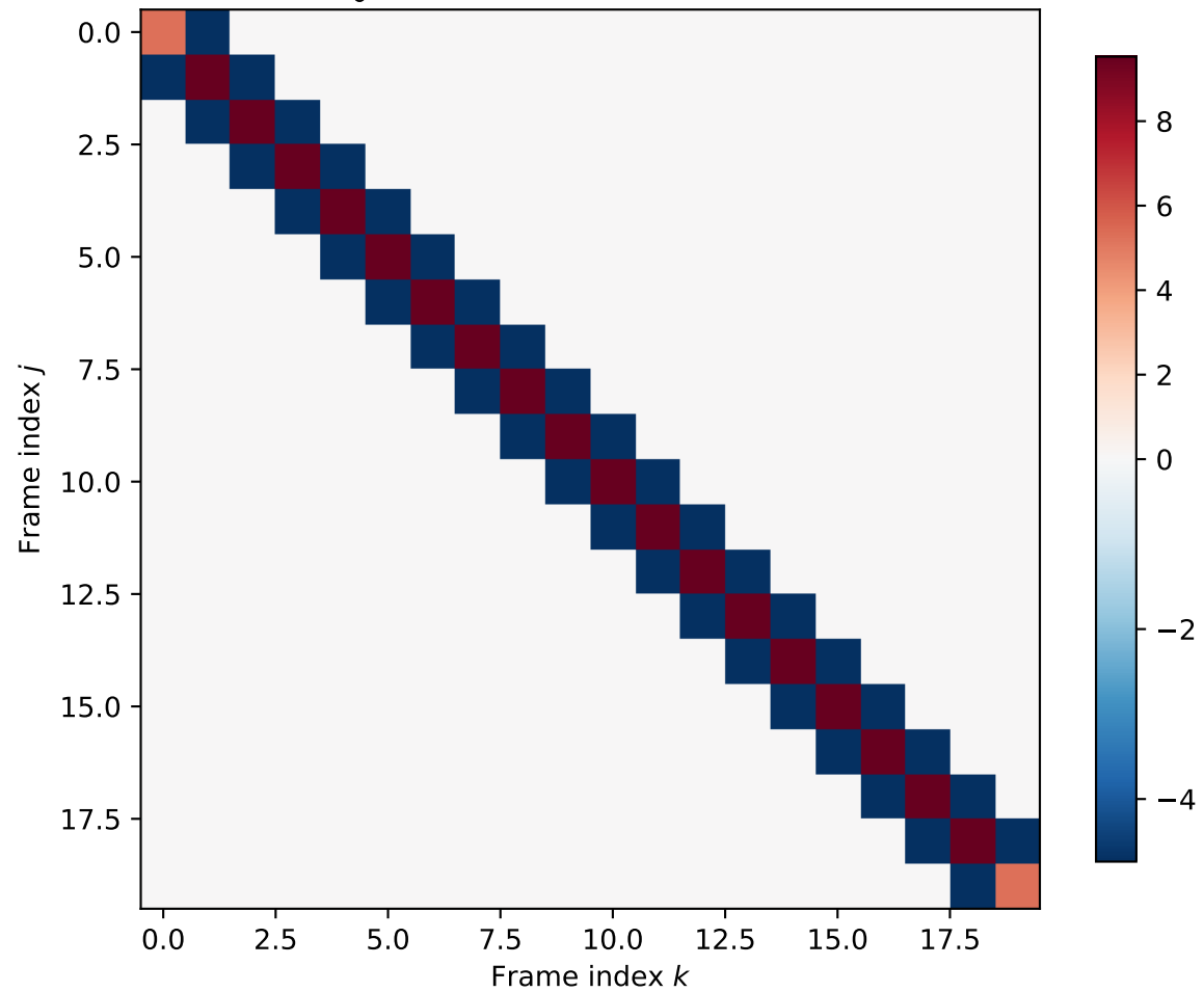
\Sigma_0^{-1} (Precision — Tridiagonal)
