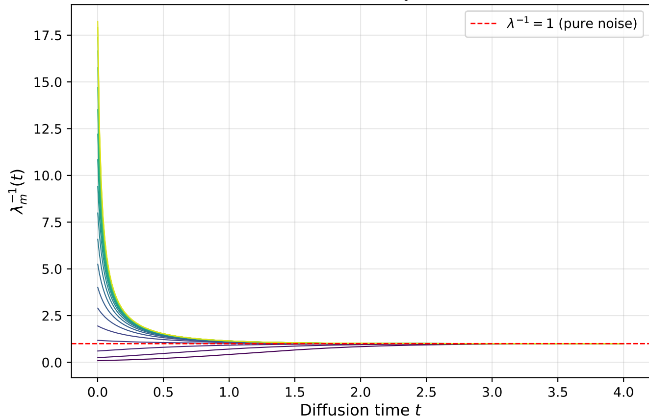
Eigenvalues of \Sigma_t^{-1} vs t
