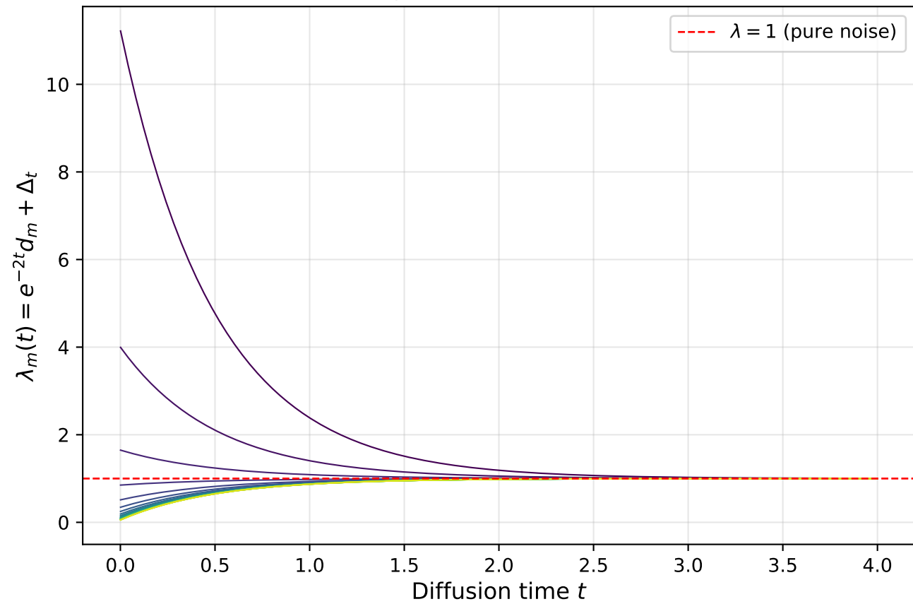
Eigenvalues of \Sigma_t vs t
